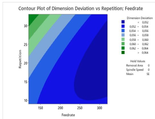
Figure 7. Contour Plot of Dimension Deviation on S-33 Machine.
