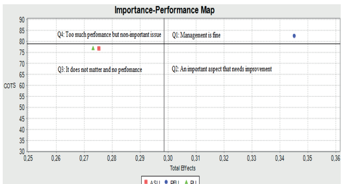
Figure 5. IPMA of Computational Thinking Skills
