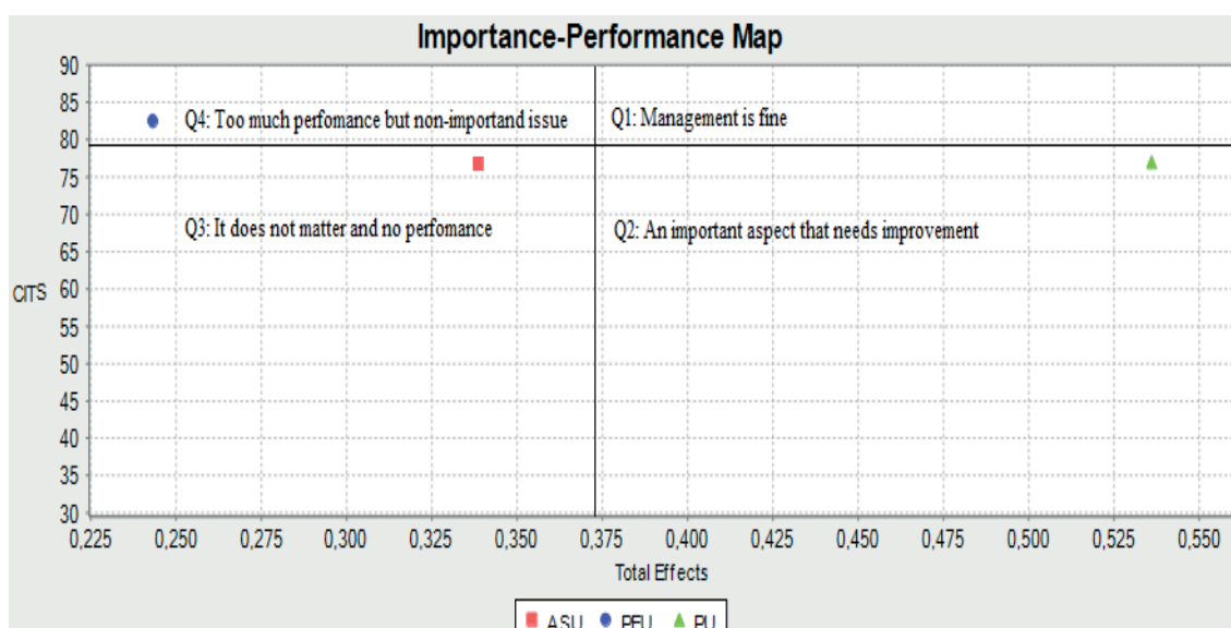
Figure 6. IPMA of Critical Thinking Skills
